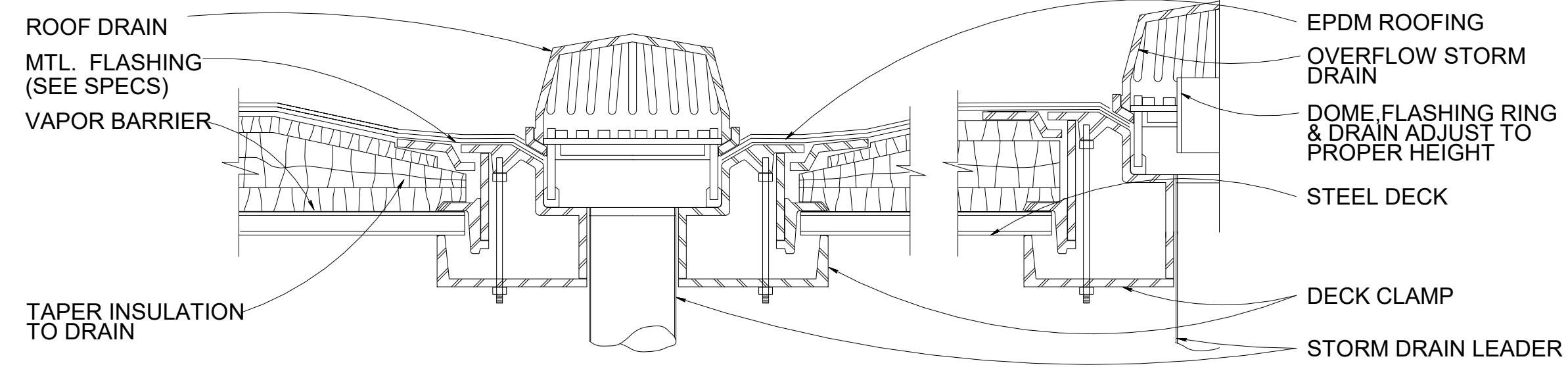
2 ROOF DRAIN DETAIL SCALE: 1/12" = 1'-0"
